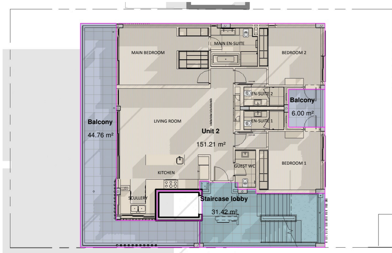
THIRD FLOOR
